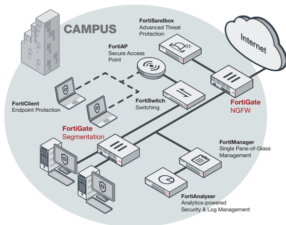
Large Campus Network Deployment (NGFW, Intent-based Segmentation)
